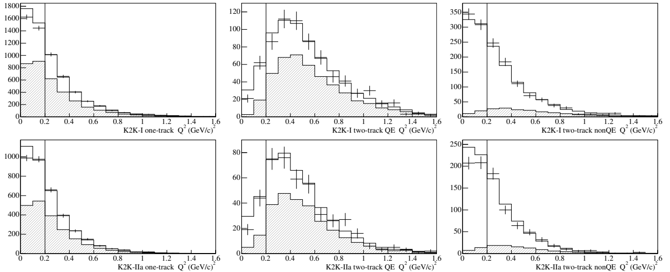
FIG. 7: The data and the best fit Q_{rec}^2 distributions for K2K-I data (top) and K2K-IIa data (bottom) for the 1-track, 2-track QE enhanced, and 2-track non-QE enhanced samples. The shaded region shows the QE fraction of each sample, estimated from the MC. The contribution from each energy region is summed for each plot. The lowest two data points in each plot are not included in the fit, due to the large uncertainty in the effects of the nucleus.
