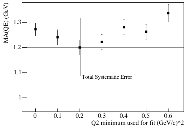
FIG. 9: Fit values obtained for different values of the low Q^2 cut. Only statistical errors are shown. The horizontal line is the combined best fit. The vertical line is the systematic errors.
